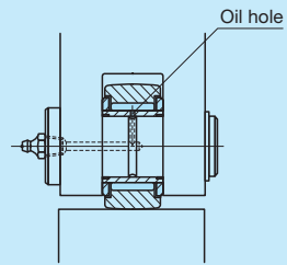
Fig. 2 Oil hole location and loading direction
