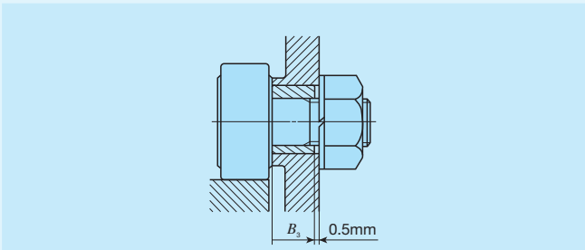
Fig. 5 Length of a mounting hole for Eccentric Type Cam Followers
