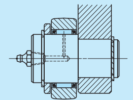
Fig. 3 Mounting examples of bearing without inner ring
