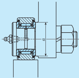
Fig. 1 Height of side surface of mounting part
